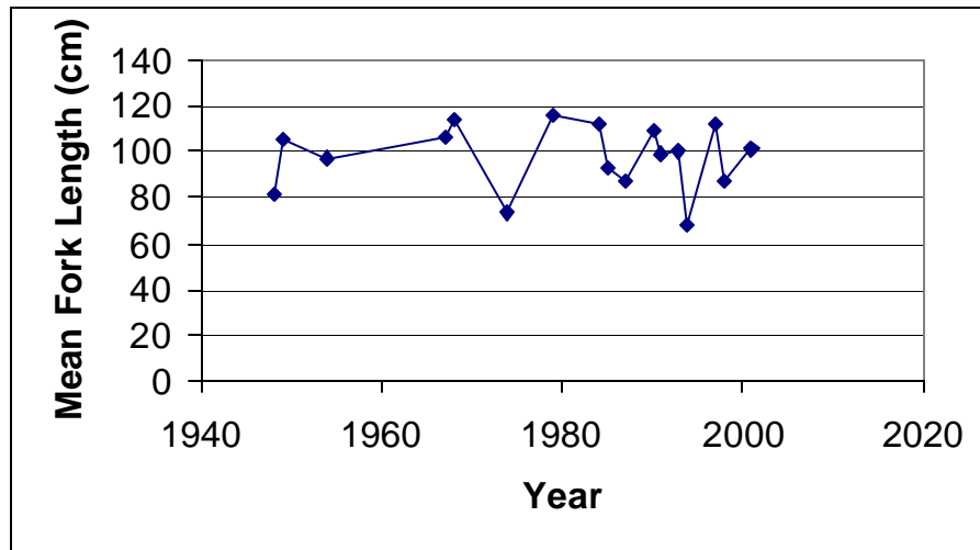
Figure 12. Green sturgeon mean fork length measured from San Pablo Bay tagging program. (n = 640, Data from CDFG 2002, TL converted to FL using conversion from Rien et al. 2001).
